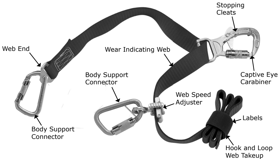
Figure 7 - Adjustable Web Lanyard
